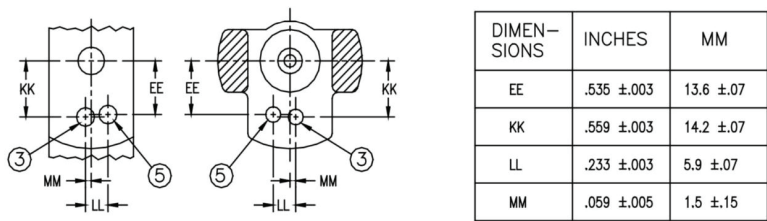
Figure 3: CGA Connection No. 910
