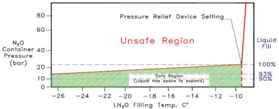
Figure 4: Safe filling volumes for 319 psi (22 bar nitrous oxide storage tanks END OF DOCUMENT
