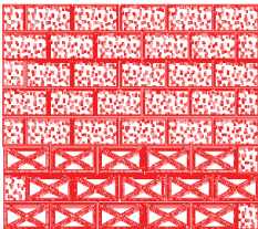
ACCEPTABLE DECORATIVE OPENBLOCK 25% of FACE AREA w/ NATURAL CROSS VENTILATION
