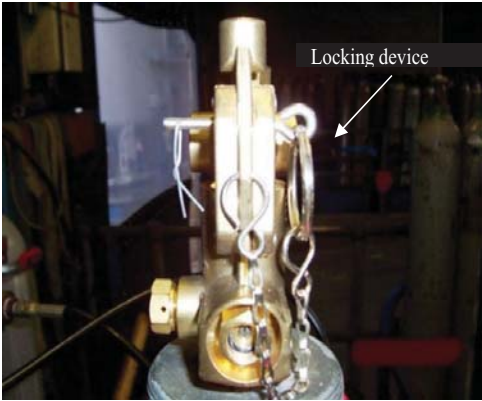
Figure 14: Quick opening cylinder valve for fire suppression system in closed position with locking device engaged
