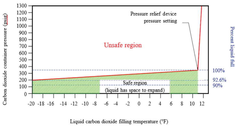
Figure 9: Safe filling volumes for 350 psi carbon dioxide containers
