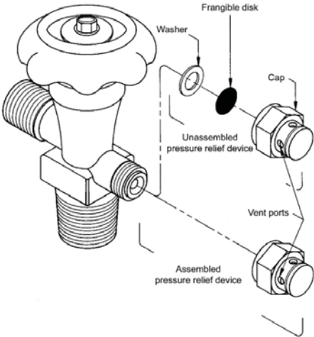
Figure 13: Carbon dioxide cylinder valve and typical pressure relief devices
