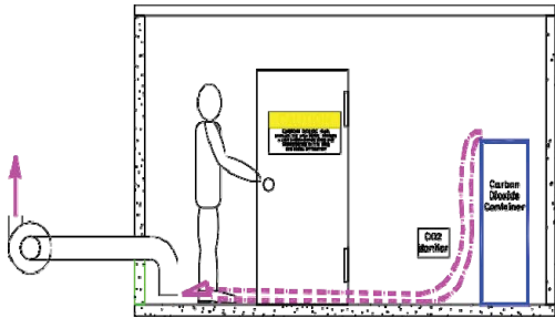
Figure 6: Example of a properly ventilated and monitored enclosed space
