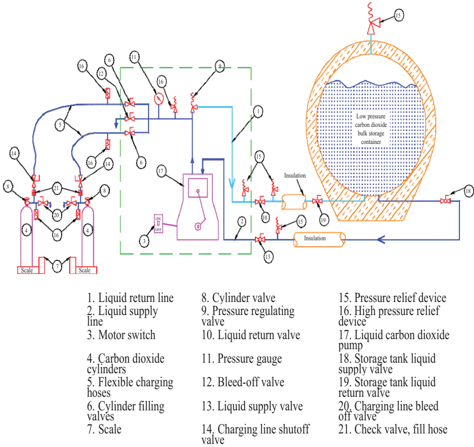
Figure 18: Typical carbon dioxide cylinder filling system schematic
