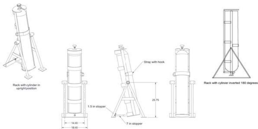
NOTE: Do not use inverting racks with siphon-type cylinders. Figure 19: Cylinder inverting
