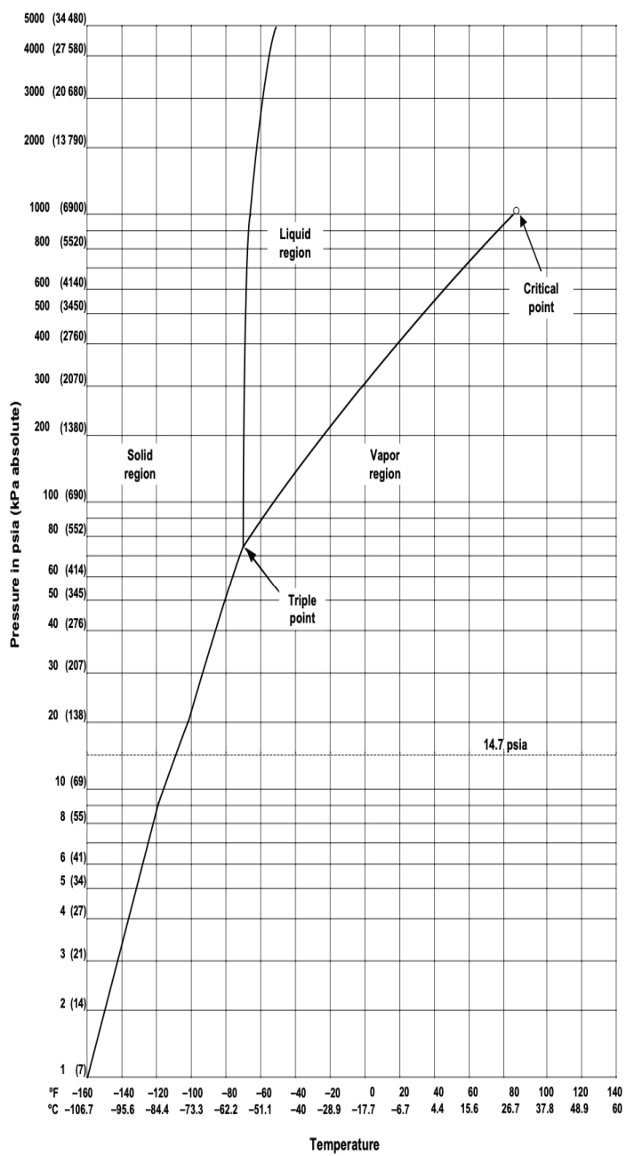
Figure 1: Carbon dioxide phase diagram
