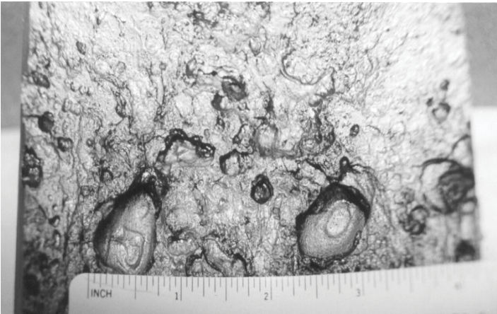
Figure 17: Sidewall corrosion of a condemned carbon dioxide cylinder
